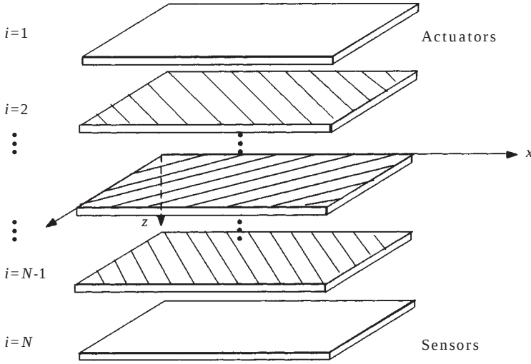
Figure 1. A typical laminated piezoelectric composite plate.
