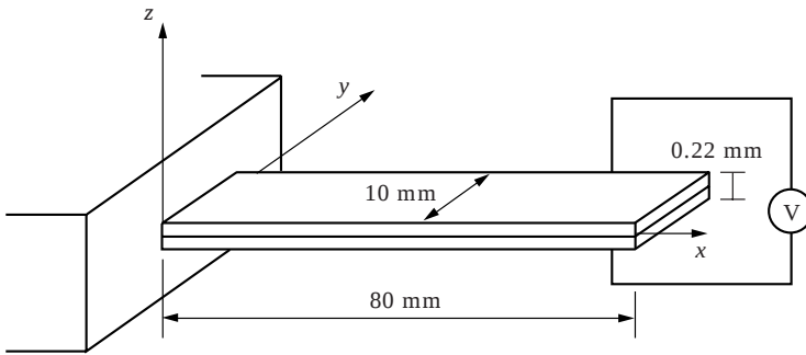
Figure 2. Piezoelectric KYNAR cantilever beam.
