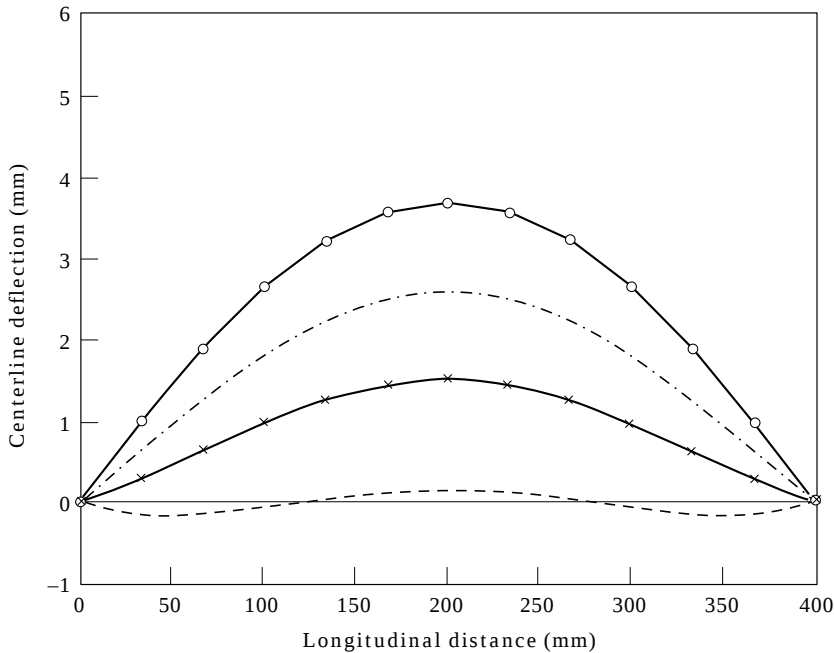
Figure 7. Centerline deflection of the plate under uniformly distributed load and different actuate voltages. \bigcirc , 0 V; - \cdot - , 40 V; \times , 80 V; - - - 130 V.
