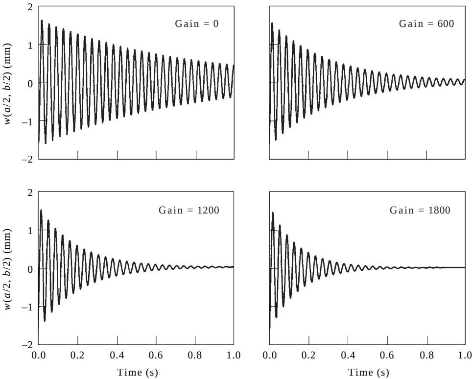
Figure 9. The effect of feedback control gain G on the plate's response.
